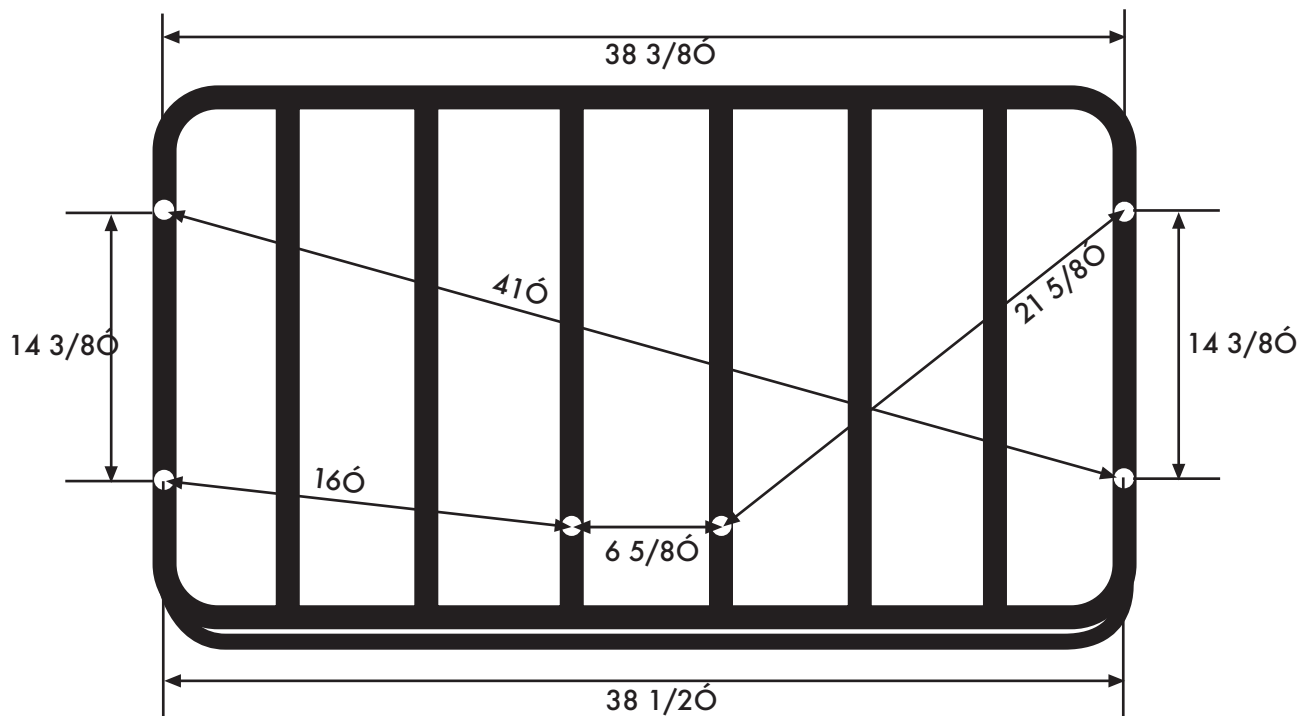
ET39B\M 6-HOLE (measurements are from center of hole)
