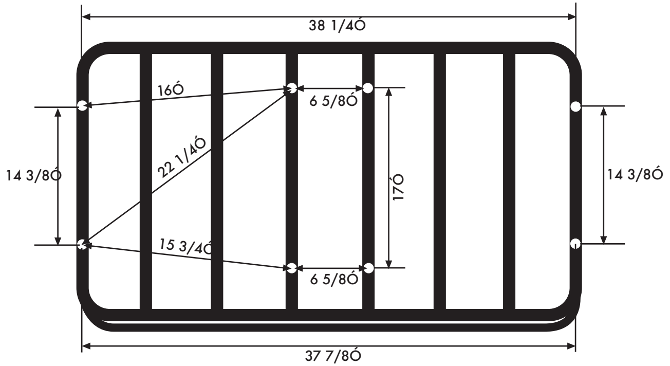
ET39D\Q 8-HOLE (measurements are from center of hole)
